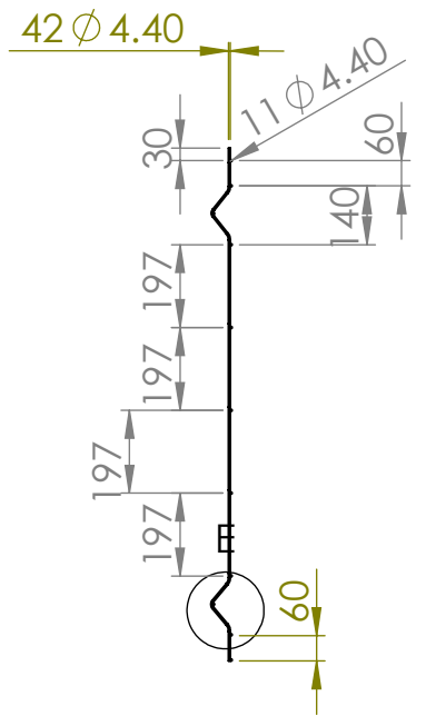
DETAIL E SCALE 1 : 10
